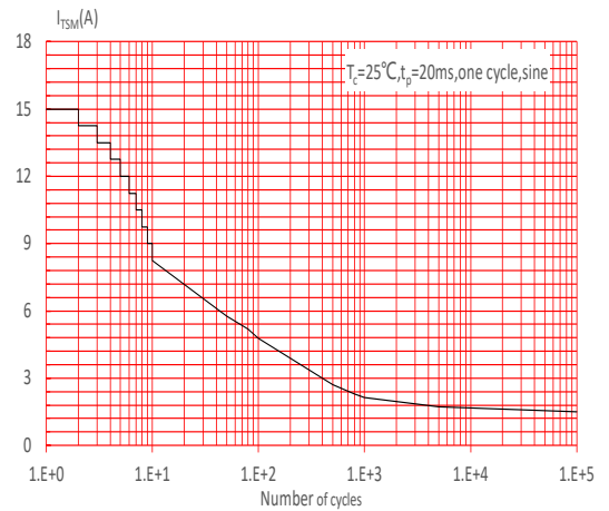
FIG.6: Non-repetitive surge peak on-state current for a sinusoidal pulse with width t_p < 20\text{ms} , and corresponding value of I^2t ( dl/dt < 50\text{A}/\mu\text{s} )
