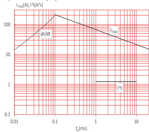
FIG.6: Non-repetitive surge peak on-state current for a sinusoidal pulse with width t_p < 20\text{ms} , and corresponding value of I^2t ( dl/dt < 50\text{A}/\mu\text{s} )
